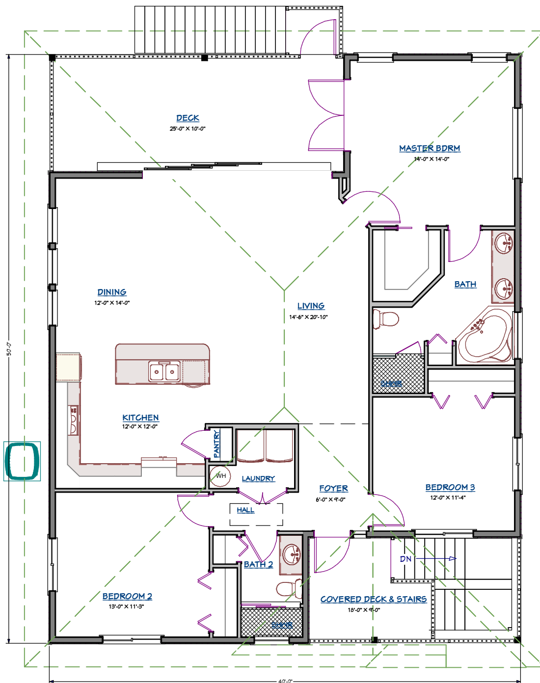
Raised Level Floor Plan
